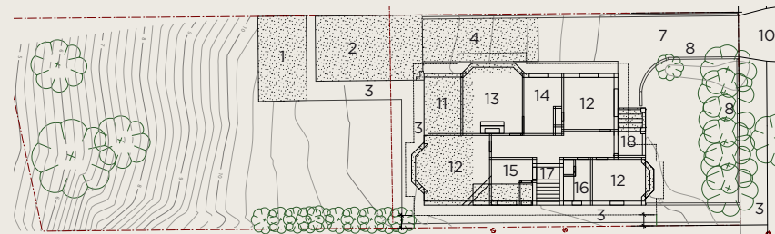
Existing top floor plan
