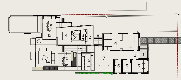
Existing basement floor plan
